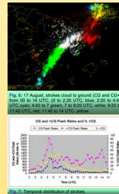
Fig. 6: 17 August, strokes cloud to ground (CG and CGF) from 00 to 14 UTC. (0 to 2:20 UTC, blue; 2:20 to 4:40 UTC cyan; 4:40 to 7 green; 7 to 9:20 UTC, white; 9:20 to 11:40 UTC, red; 11:40 to 14 UTC, yellow).
